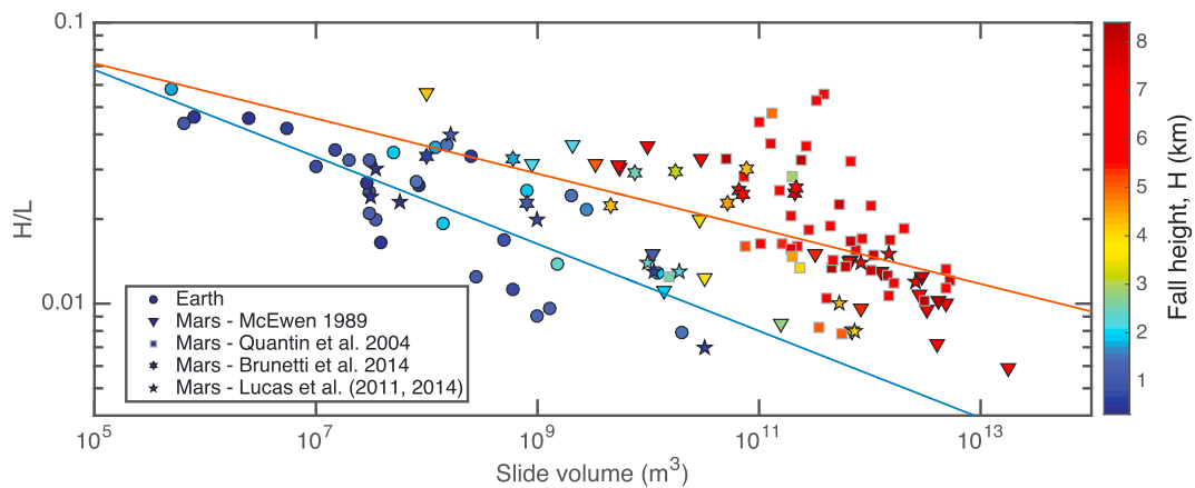
Figure 1. H/L versus slide volume of observed terrestrial and Martian landslides. Observed terrestrial (Legros, 2002) (circles) and Martian (McEwen, 1989) (triangles), (Quantin et al., 2004) (squares), (Brunetti et al., 2014) (hexagram), and (Lucas et al., 2011, 2014) (pentagram) colored by fall height H according to the color bar. The red and blue trend lines are based on Martian and terrestrial observations, respectively.
