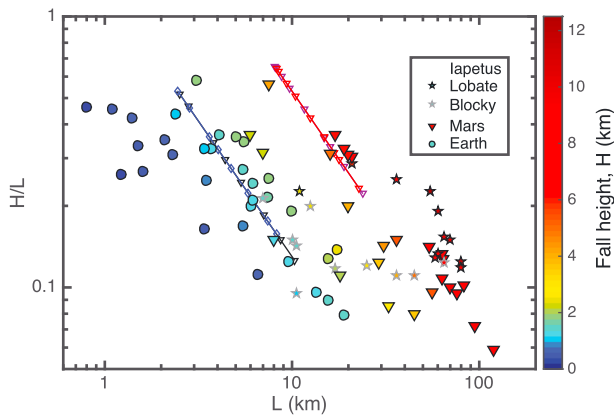
Figure 4. Comparison of H/L versus L . Observed landslides on Earth (Legros, 2002) (circles), Mars (McEwen, 1989) (triangles), and Iapetus (Singer et al., 2012) (pentagram) colored by fall height H according to the color bar. The lines are simulation results reported in Figure 3.
