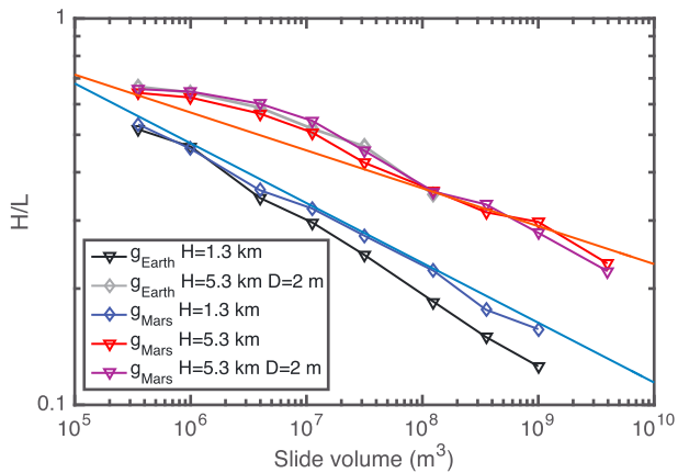
Figure 3. H/L versus slide volume of simulated terrestrial and Martian landslides. Simulations for different fall heights, surface gravities, and particle sizes as indicated in the legend (the black triangles were previously reported in by Johnson et al., 2016). Each point represents the result of a single simulation. Trend lines for observed terrestrial and Martian slides from Figure 1 are included for comparison.
