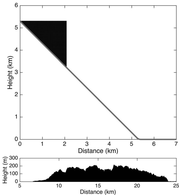
Figure 2. (top) Initial and (bottom) final slide geometry for 5.3 km fall height D = 2 m and Martian gravity. The black points mark the location of individual particles. The thick gray curve in the top plot shows the ground contour. Note that the bottom plot is 10 times vertically exaggerated.
