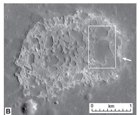
Figure 1. A: Ina shield volcano on the Moon; Lunar Orbiter Laser Altimeter (LOLA) topography overlying Kaguya Terrain Camera mosaic TCO_MAPe04_N21E003N18E006SC, 25 m contour interval. Top: West-east elevation profile (a-a'), ~22.6× VE (vertical exaggeration). B: Ina pit crater, showing mounds (gray) and hummocky and/or blocky floor units; Lunar Reconnaissance Orbiter Camera Narrow Angle Camera M119815703, 0.48 m/pixel, ~56° incidence angle. White rectangle marks location of Figure 2B; white arrow shows viewing direction of Figure 2A.
