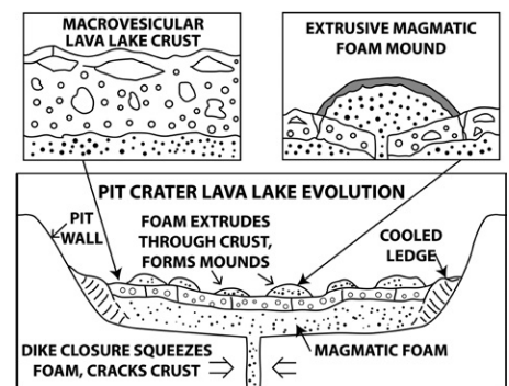
Figure 3. Cross section of the waning stage process of magmatic foam emplacement in the Ina summit pit crater (Moon).
